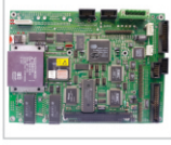
Mother Board
